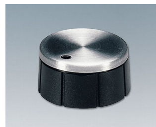
A1624260 TUNING KNOB, with lateral screw fixing ABS (UL 94 HB) black/alu 24x12,4mm 6mm
