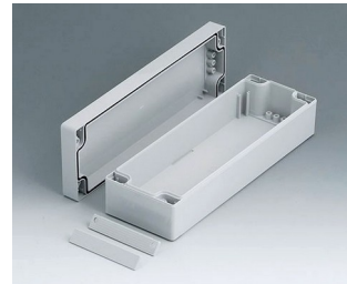
C2008241 ROBUST-BOX 80 BREIT, Ausf. I ABS (UL 94 HB) lichtgrau RAL 7035 240x80x60mm IP 66
