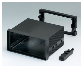
B6032021 DIN-MODULAR CASE TYPE A, Vers. I PPO (UL 94 V-0) black RAL 9005 96x48x75mm
