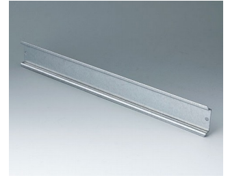
C7118077 Standard DIN rail, Type TH 35 Steel 283,5x35x7,5mm
