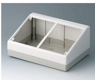
A9082065 DESK CASE 220 ABS (UL 94 HB) off-white RAL 9002 220x156x100mm
