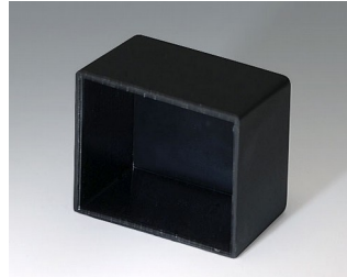
A8017108 POTTING BOXES, Vers. III PA 66 (UL 94 V-2) black RAL 9005 17.4x15x10.5mm
