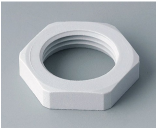
C2320117 Counter nut M20x1.5 PA light grey RAL 7035
